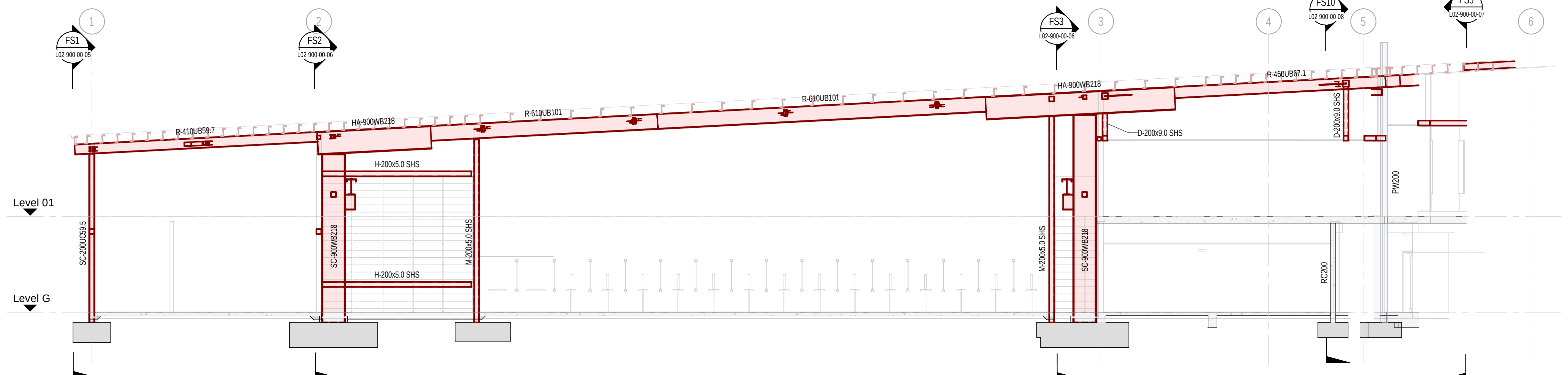
SECTION PF10 SCALE 1:100 102-510-00-02
