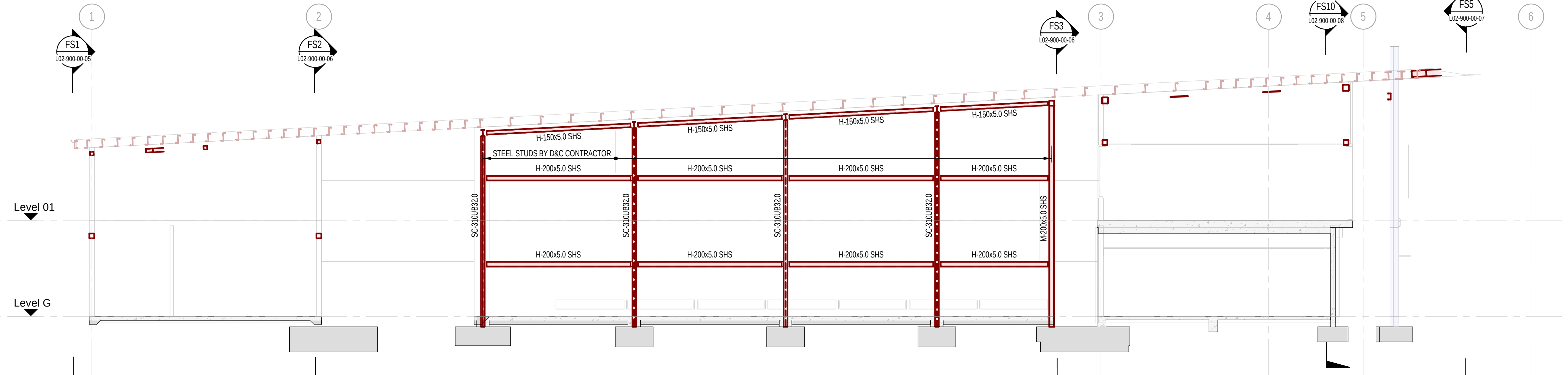
SECTION FSD SCALE 1:100 L02-510-00-02
