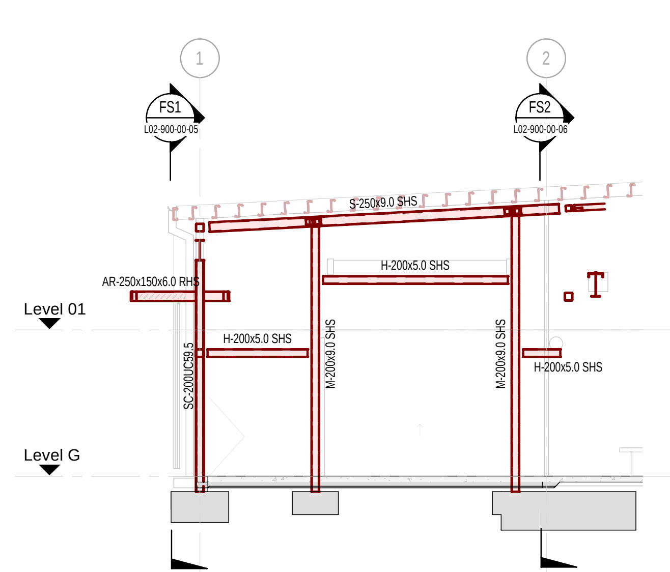
SECTION FS16 SCALE 1 : 100 L02-510-00-02
